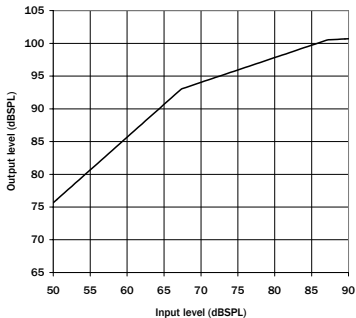
FIGURE 2. Input/Output Function @ 2000 Hz
