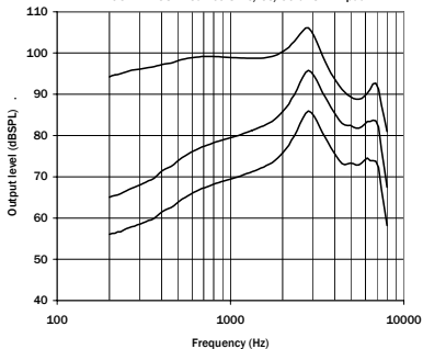
FIGURE 1. OSPL Curves @ 50/60/90 dB SPL Input
